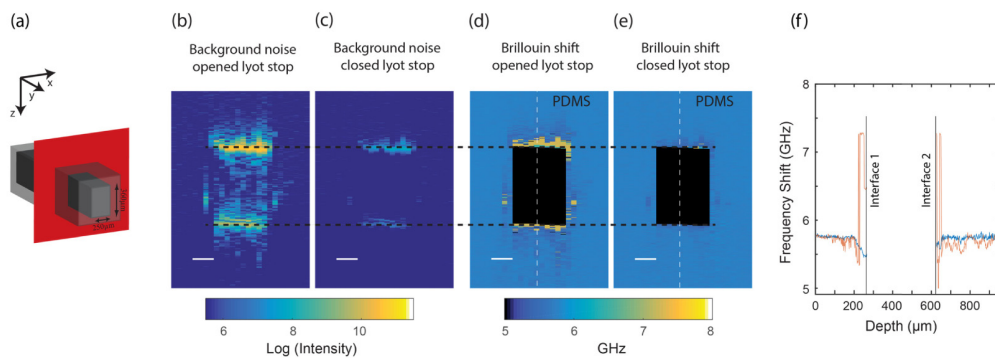
Fig. 4. Brillouin imaging of a micro-fluidic channel: (a) Illustration of the PDMS micro fluidic channel (width = 250 \mu\text{m} , height = 360 \mu\text{m} ). Scanning was performed across the XZ plane highlighted in red. Background noise levels defined as the average intensity value between the Brillouin peaks with (b) the Lyot stop widely open and (c) with a closed Lyot stop (scale bar = 100 \mu\text{m} ). The noise from the interfaces was nearly removed for the latter. False color bar indicates camera counts on log scale. Brillouin shifts recorded with (d) an open Lyot stop and (e) a closed Lyot stop. For the former there are clear artifacts up to 50 microns away from the interfaces, whereas the latter show a continuous Brillouin shift up to the interface between air and PDMS. (f) Line plots of the Brillouin shift measurements across the central part of microfluidic channel denoted by a dashed line in Figs. 4(d) and 4(e), for an opened Lyot stop (red) and a closed Lyot stop (blue).
