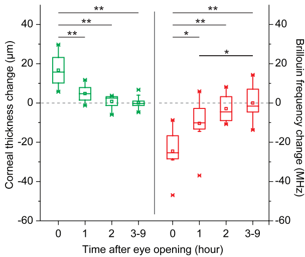
FIGURE 5. CCT change ( \Delta\text{CCT} ) and Brillouin frequency change ( \Delta\Omega ) in the hours following eye-opening in the morning. The reference points for these changes are the mean values measured over 3 to 9 hours after waking. * P < 0.01 , ** P < 0.05 .
